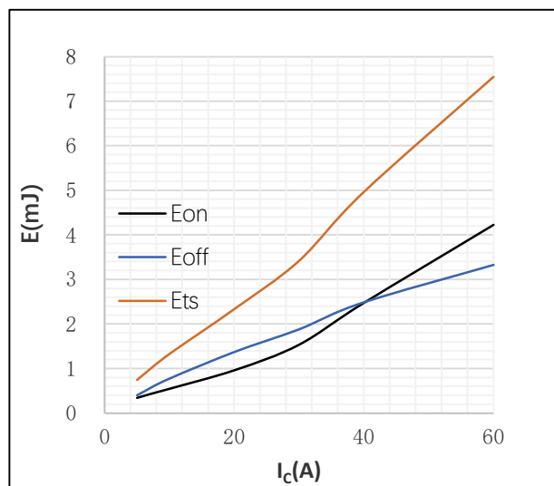
● Fig.17 Switching energy losses as a function of collector current; typical values
