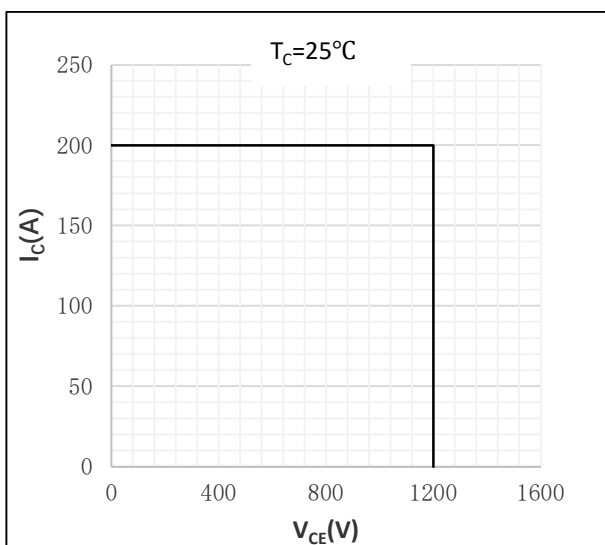
● Fig.15 Reverse bias safe operating area: peak collector currents as a function of collector-emitter voltage; Calculative values
